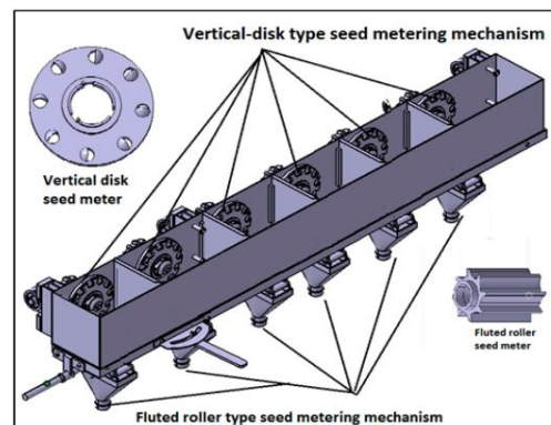
Figure 2. Seed box with vertical disk and fluted roller type seed metering mechanisms.
